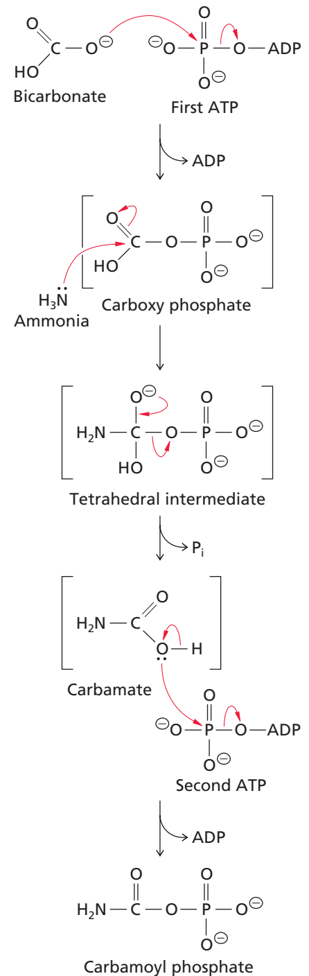
▲ Figure 17.41 Synthesis of carbamoyl phosphate catalyzed by carbamoyl phosphate synthetase I. The reaction involves two phosphoryl-group transfers. First, nucleophilic attack by bicarbonate on ATP produces carboxy phosphate and ADP. Next, ammonia reacts with carboxy phosphate, forming a tetrahedral intermediate. Elimination of a phosphate group produces carbamate. A second phosphoryl-group transfer from another ATP forms carbamoyl phosphate and ADP. Structures in brackets remain enzyme bound during the reaction.
