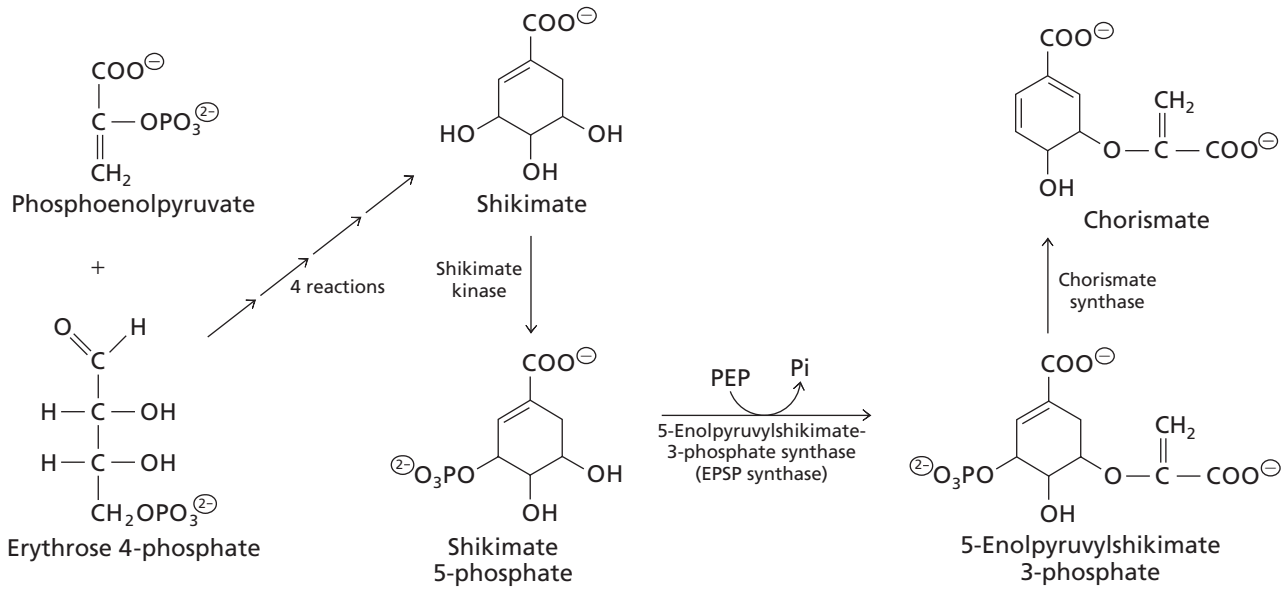
▲ Figure 17.19 Synthesis of shikimate and chorismate.
