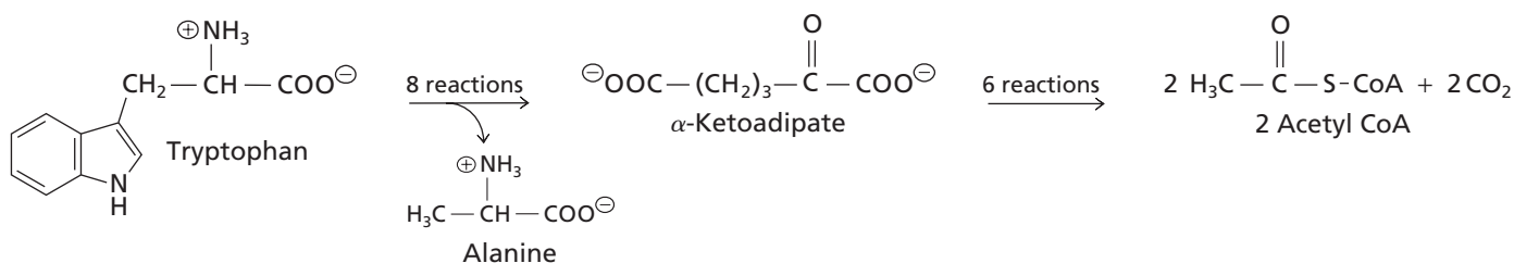
▲ Figure 17.38 Conversion of tryptophan to alanine and acetyl CoA.
