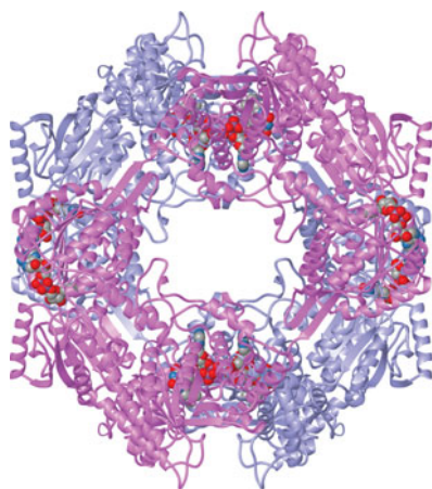
▲ Proline utilization A flavoprotein. This enzyme from Bradyrhizobium japonicum combines the first two enzymes in the proline degradation pathway into a large complex consisting of six subunits of bifunctional proteins. The two identical subunits of one core dimer are colored blue and purple and the entire structure consists of three such dimers arranged in a circle. The bound FAD and NAD + coenzymes are shown as space-filling models. This enzyme presumably confers a selective advantage over species containing two separate enzymes so why hasn't it evolved in eukaryotes? [PDB 3HAZ]
