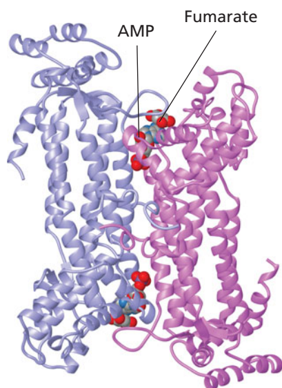
▲ Adenylosuccinate lyase from E. coli . The enzyme is a homodimer. One subunit is colored blue and the other is purple. This is a mutant enzyme (H171N) showing the two products, AMP and fumarate, bound at the active sites. Adenylosuccinate lyase catalyzes similar steps in the IMP synthesis pathway and in the conversion of IMP to AMP. [PDB 2PTQ]
