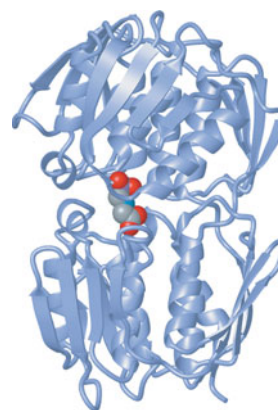
▲ E. coli 5-enolpyruvylshikimate-3-phosphate synthase with a molecule of glyphosate bound to the active site. [PDB 2AAY]
