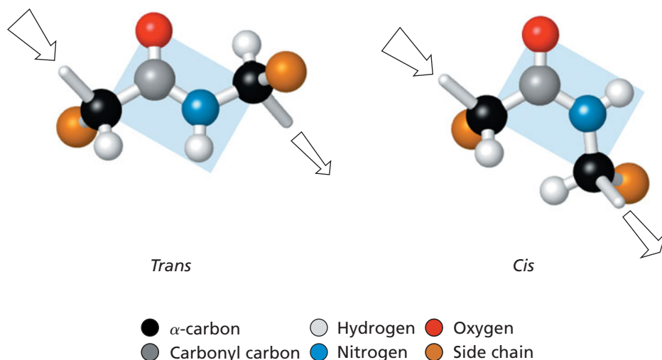
◀ Figure 4.7 Trans and cis conformations of a peptide group. Nearly all peptide groups in proteins are in the trans conformation, which minimizes steric interference between adjacent side chains. The arrows indicate the direction from the N- to the C-terminus.
