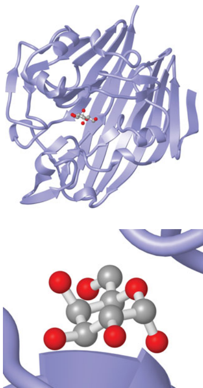
▲ Galactose mutarotase. Mutarotases are enzymes that catalyze the interconversion of \alpha and \beta configurations. This interconversion involves the breaking and remaking of covalent bonds, which is why they are different configurations. The enzyme shown here is galactose mutarotase from Lactococcus lactis with a molecule of \alpha -D-galactose in the active site. The bottom figure shows the conformation of this molecule. Can you identify this conformation? [PDB 1L7K]
