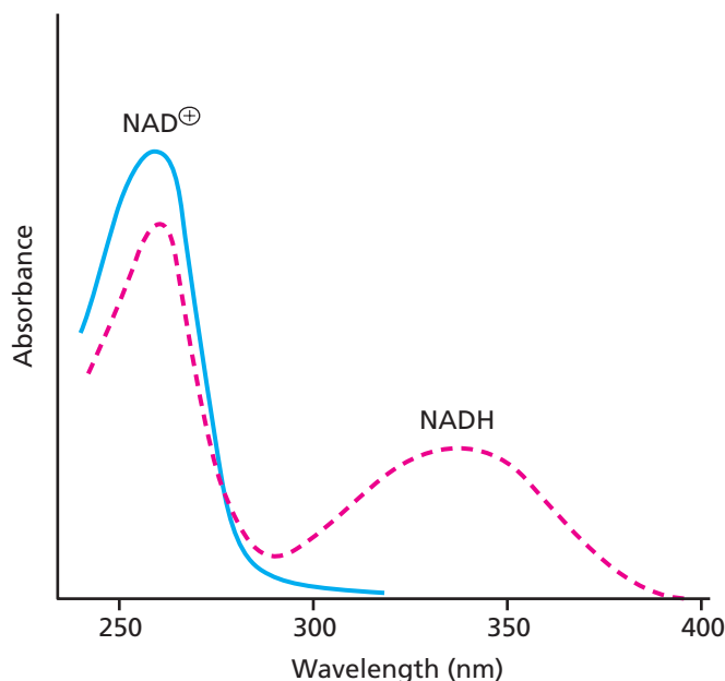
▲ Ultraviolet absorption spectra of NAD + and NADH.
