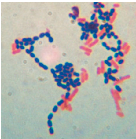
▲ The Gram stain. The Gram staining procedure distinguishes between gram-positive bacteria (left, purple) and gram-negative bacteria (right, pink).
