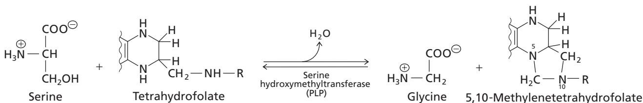
▼ Figure 17.16 Biosynthesis of glycine.
