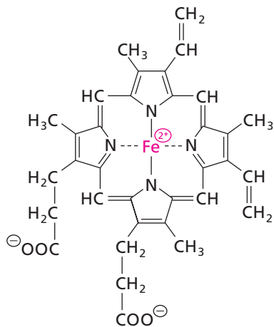
▲ Figure 4.45 Chemical structure of the Fe(II)-protoporphyrin IX heme group in myoglobin and hemoglobin. The porphyrin ring provides four of the six ligands that surround the iron atom.
