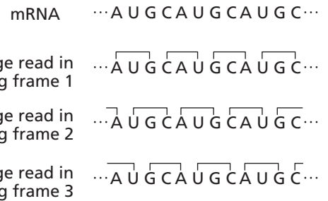
▲ Figure 22.2 One mRNA contains three different reading frames. The same string of letters read in three different reading frames will be translated into three different “messages” or protein sequences. Thus, translation of the correct message requires selecting the correct reading frame.
