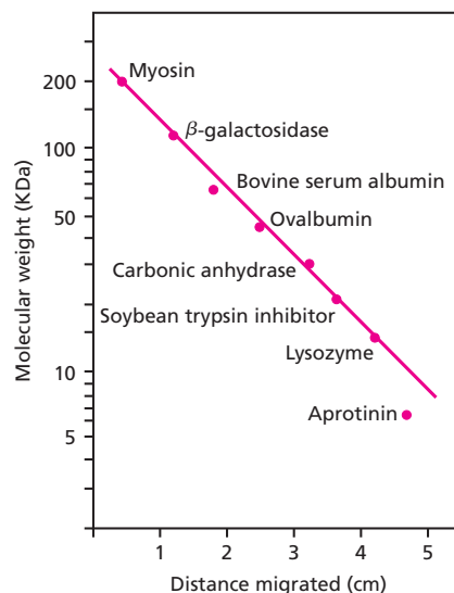
▲ Figure 3.13 Proteins separated on an SDS–polyacrylamide gel. (a) Stained proteins after separation. The high molecular weight proteins are at the top of the gel. (b) Graph showing the relationship between the molecular weight of a protein and the distance it migrates in the gel.
