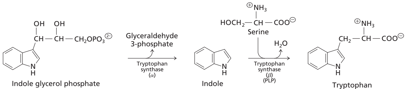
▲ Figure 17.22 Reactions catalyzed by tryptophan synthase.
