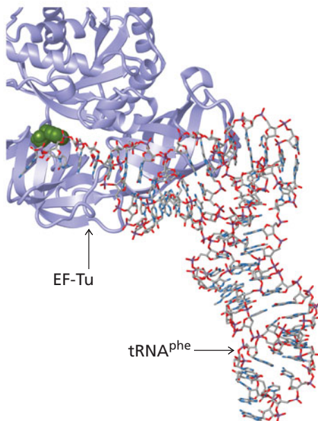
▲ Figure 22.20 EF-Tu binds aminoacylated tRNAs. The EF-Tu-GTP complex binds to the acceptor end of aminoacylated tRNA (in this case phenylalanyl-tRNA Phe ). The phenylalanine residue is shown in green. This is how charged tRNAs commonly exist inside a cell.
