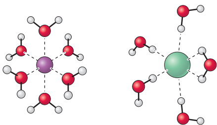
▲ Figure 2.6 Dissolution of sodium chloride (NaCl) in water. (a) The ions of crystalline sodium chloride are held together by electrostatic forces. (b) Water weakens the interactions between the positive and negative ions and the crystal dissolves. Each dissolved \text{Na}^+ and \text{Cl}^- is surrounded by a solvation sphere. Only one layer of solvent molecules is shown. Interactions between ions and water molecules are indicated by dashed lines.
