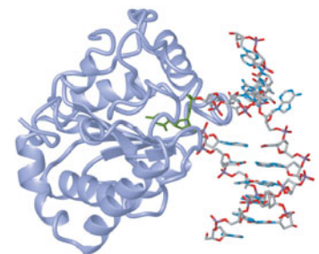
▲ Figure 20.23 Uracil N -glycosylase from human mitochondria. The enzyme is bound to a uracil-containing nucleotide (green) that has been flipped out of the stacked region of double-stranded DNA. [PDB 1EMH].
