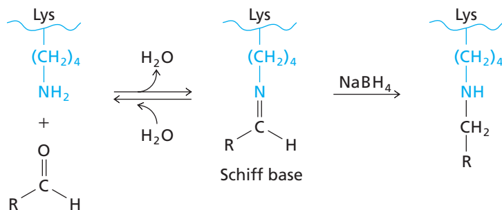
▲ Figure 5.14 Reaction of the \epsilon -amino group of a lysine residue with an aldehyde. Reduction of the Schiff base with sodium borohydride ( \text{NaBH}_4 ) forms a stable substituted amine.
