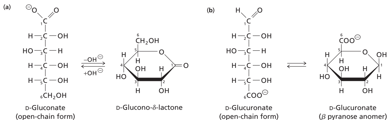
▲ Figure 8.18 Structures of sugar acids derived from D-glucose. (a) Gluconate and its \delta -lactone. (b) The open-chain and pyranose forms of glucuronate.
