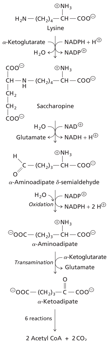
▲ Figure 17.39 Conversion of lysine to acetyl CoA.
