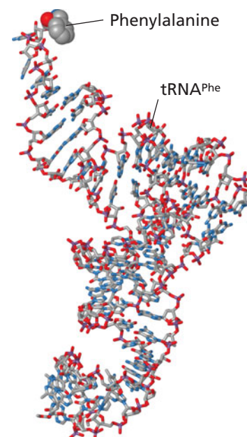
▲ Phenylanyl-tRNA Phe . Most newly synthesized amino acids are rapidly attached to their corresponding tRNAs and used in protein synthesis. [PDB 1TTT]
