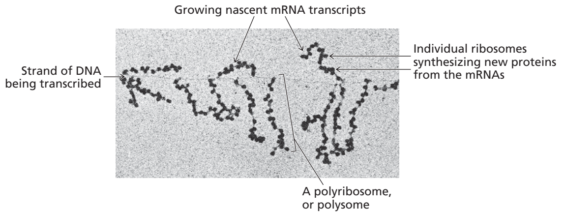
▲ Figure 22.19 Coupled transcription and translation of an E. coli gene. The gene is being transcribed from left to right. Ribosomes bind to the 5' end of the mRNA molecules as soon as they are synthesized. The large polysomes on the right are released from the gene when transcription terminates.
