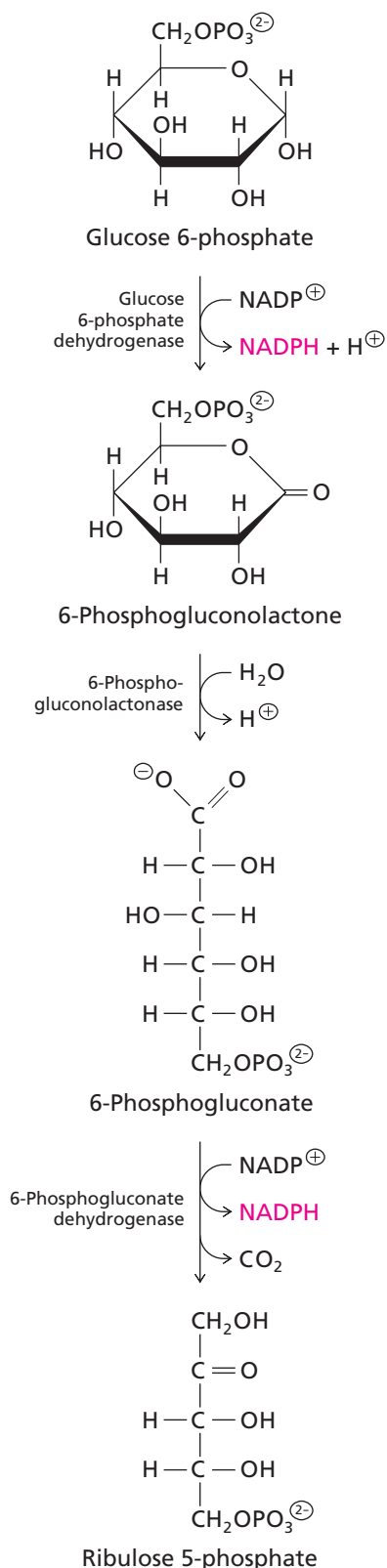
▲ Figure 12.11 Oxidative stage of the pentose phosphate pathway. Two molecules of \text{NADP}^+ are reduced to two molecules of \text{NADPH} for each molecule of glucose 6-phosphate that enters the pathway.
