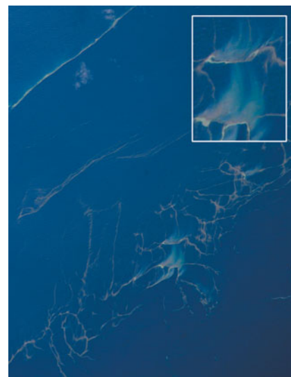
▲ Blooms of Trichodesmium . Trichodesmium is one of the main nitrogen-fixing species of cyanobacteria. This large bloom of bacteria formed giant streaks in the ocean off the coast of Australia. The photograph was taken from the space shuttle. The average concentration of nitrogen-fixing bacteria in the ocean is about one million cells per liter.
