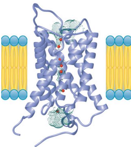
◀ Figure 9.32 Fungal aquaporin. Aquaporin is an integral membrane protein with an \alpha -helix bundle domain. The water channel (green dots) is open on the exterior surface and narrows to a tiny passage on the cytoplasmic side. [ Pichia pastoris PDB 2W2E]
