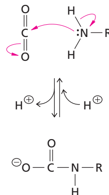
▲ Figure 4.56 Carbamate adduct. Carbon dioxide produced by metabolizing tissues can react reversibly with the N-terminal residues of the globin chains of hemoglobin, converting them to carbamate adducts.
