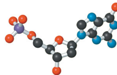
▲ Figure 19.10 Deoxyguanosine-5'-monophosphate (dGMP). Hydrogen atoms have been omitted for clarity. Color key: carbon, black; nitrogen, blue; oxygen, red; phosphorus, purple.
