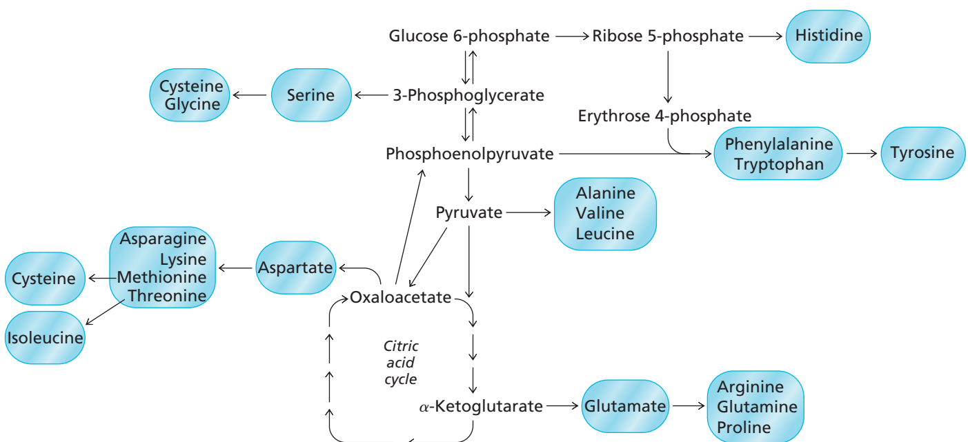
▼ Figure 17.9 Biosynthesis of amino acids, showing the connections to glycolysis/gluconeogenesis and the citric acid cycle.
