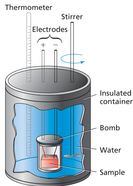
▲ The heat given off during a reaction can be determined by carrying out the reaction in a sensitive calorimeter.
