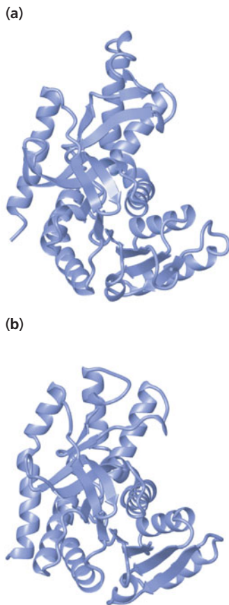
▲ Figure 4.23 Structural similarity of lactate and malate dehydrogenase. (a) Bacillus stercophilus lactate dehydrogenase [PDB 1LDN]. (b) Escherichia coli malate dehydrogenase [PDB 1EMD].
